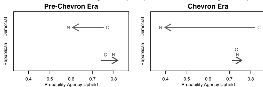
Figure 8: Predicted Probabilities
